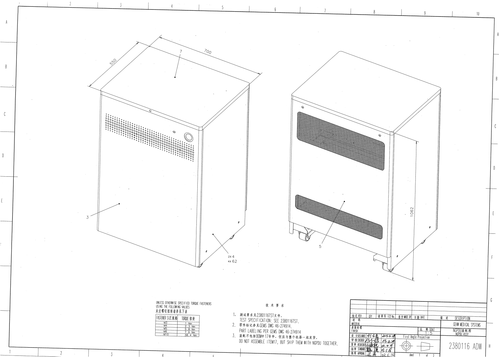
Figure 3-2 NGPDU ASSEMBLY3 (2380116ADW, sheet 1, rev 0)
